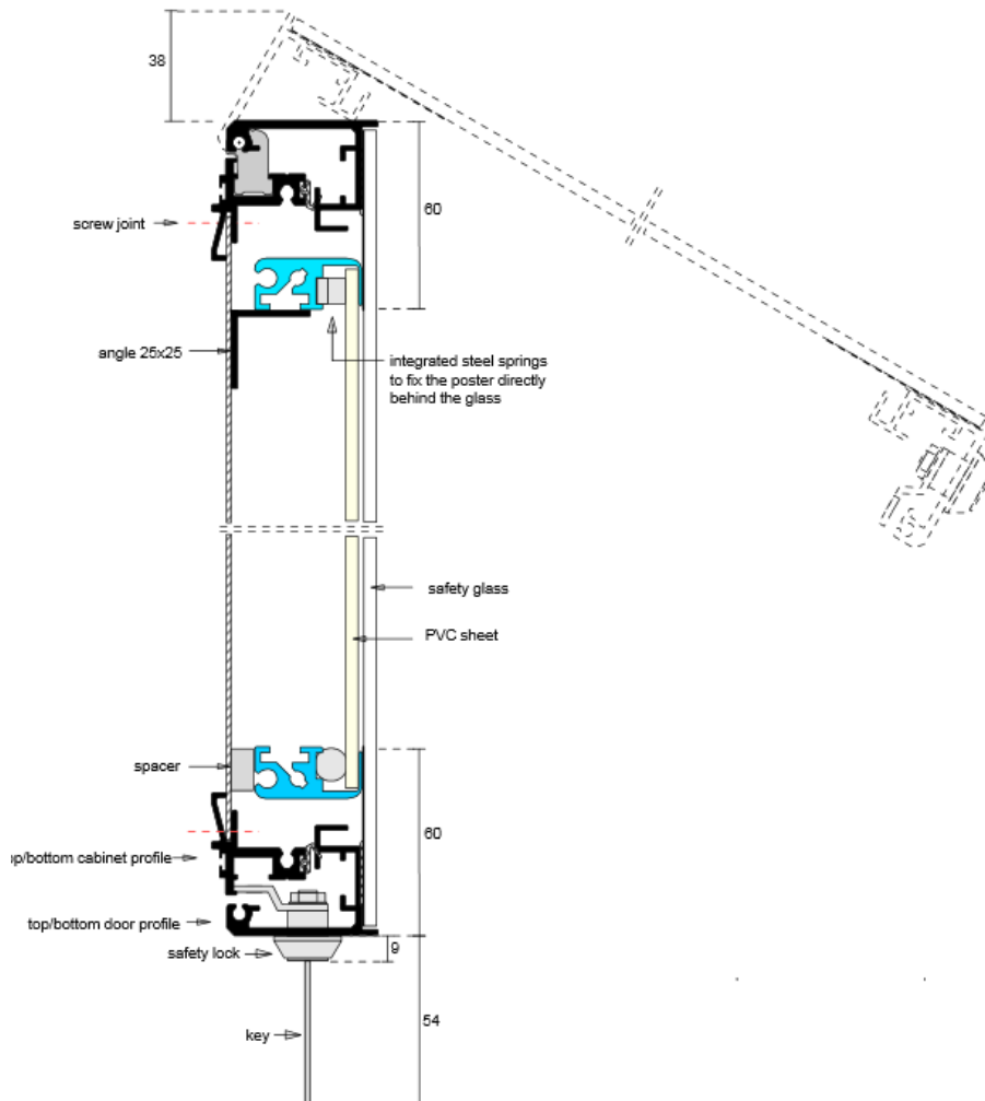
Top hinged Vitrum 400
